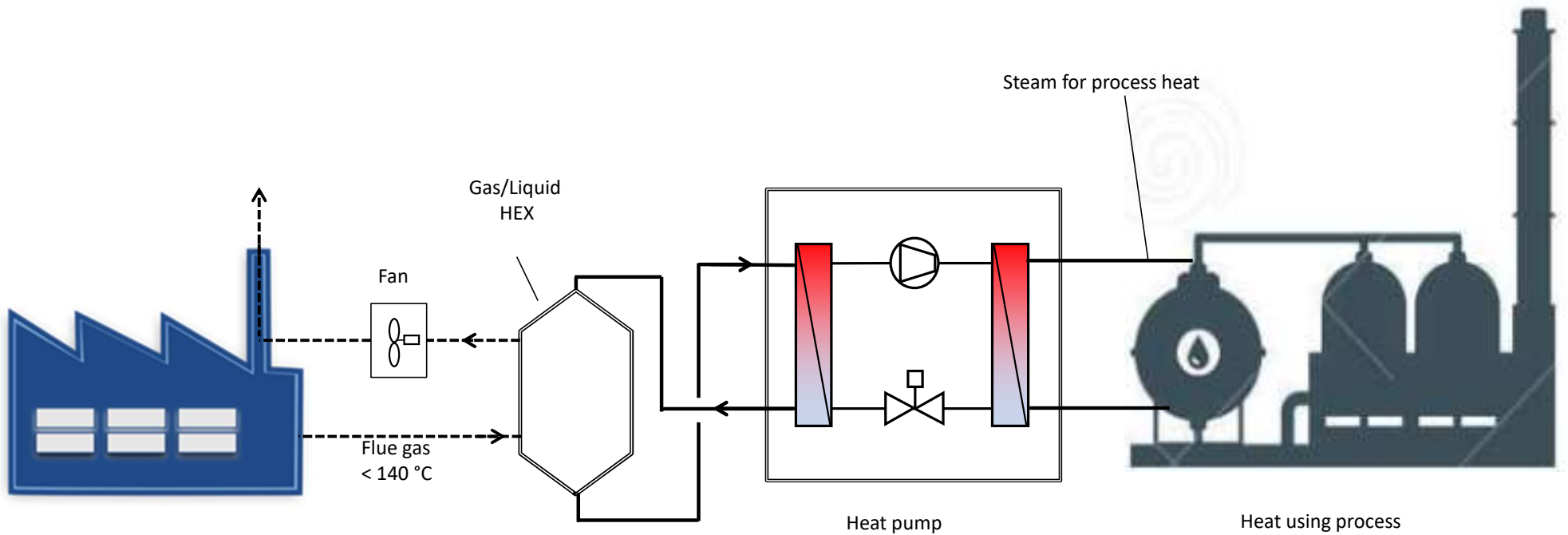
Example of steam production with a heat pump
