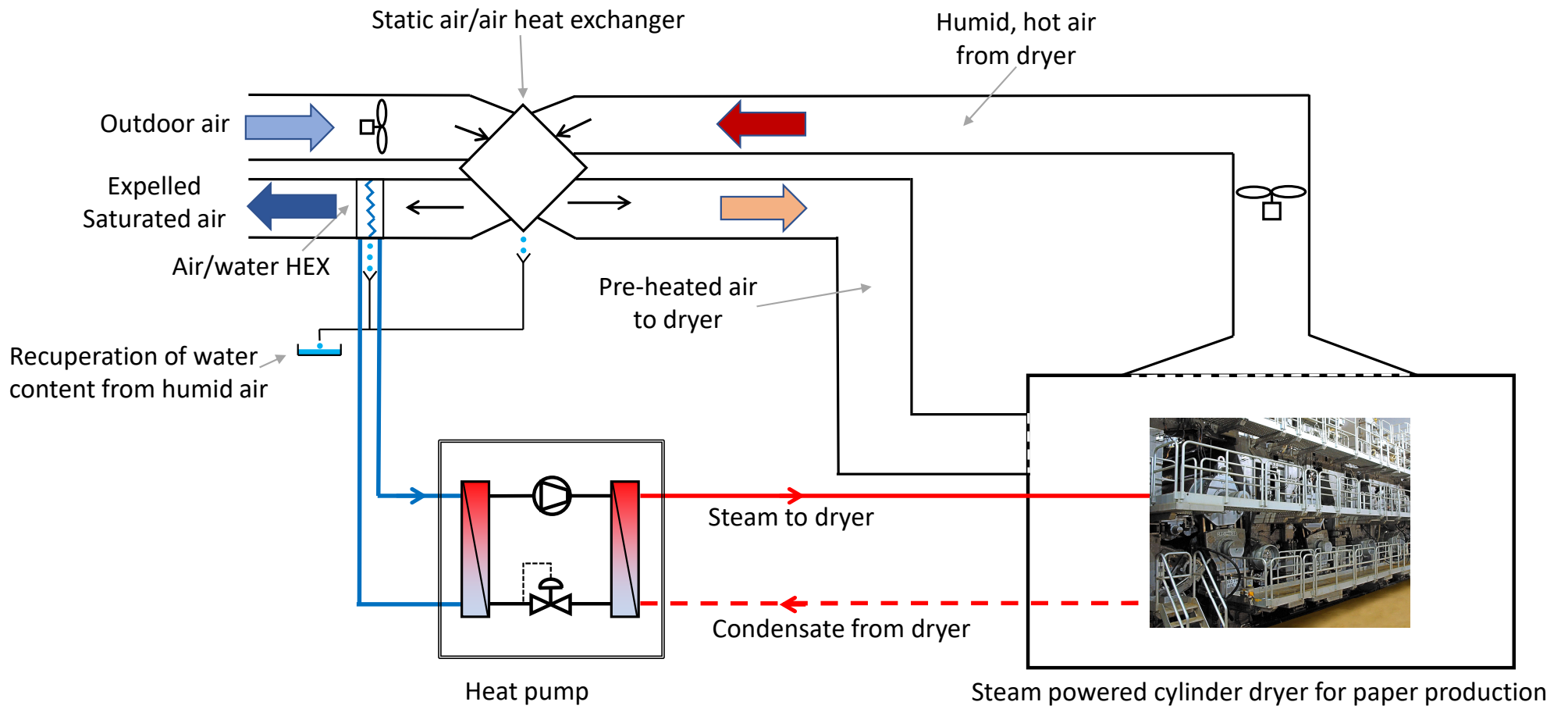
Steam production with a heat pump for the enhancement of a drying process
