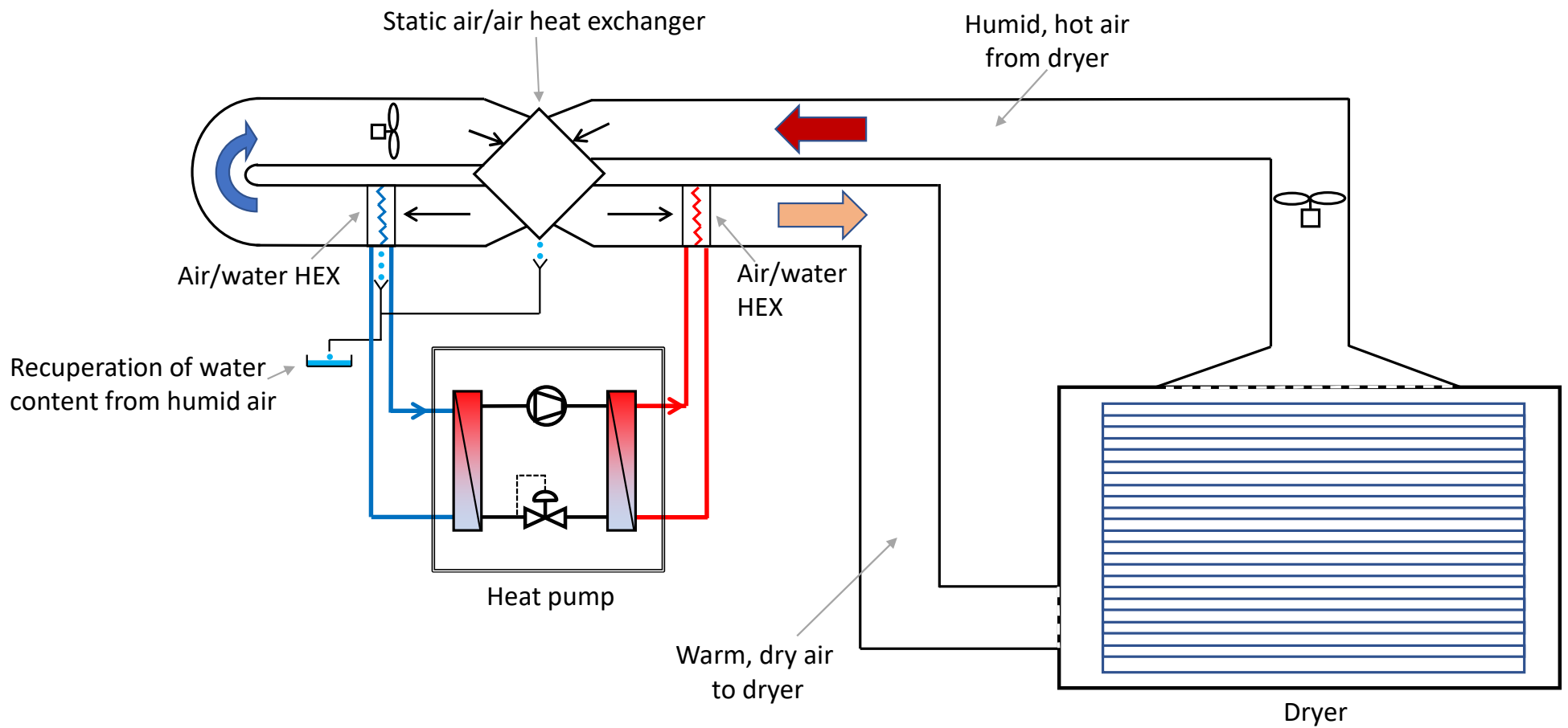
Closed loop dryer with a heat pump
