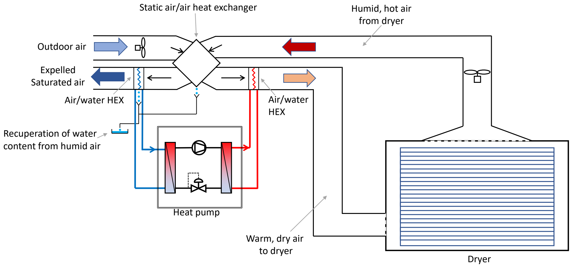
Schematic view of a heat pump for the enhancement of a drying process
